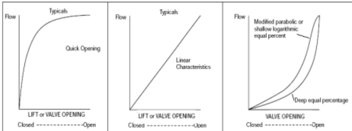
Response curve of various valves
