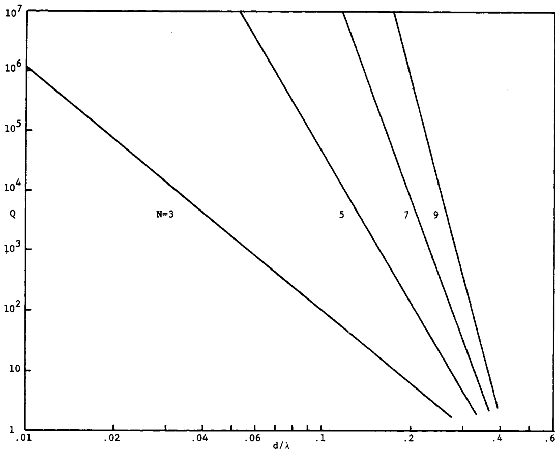
Fig. 3. Q of broadside arrays.
