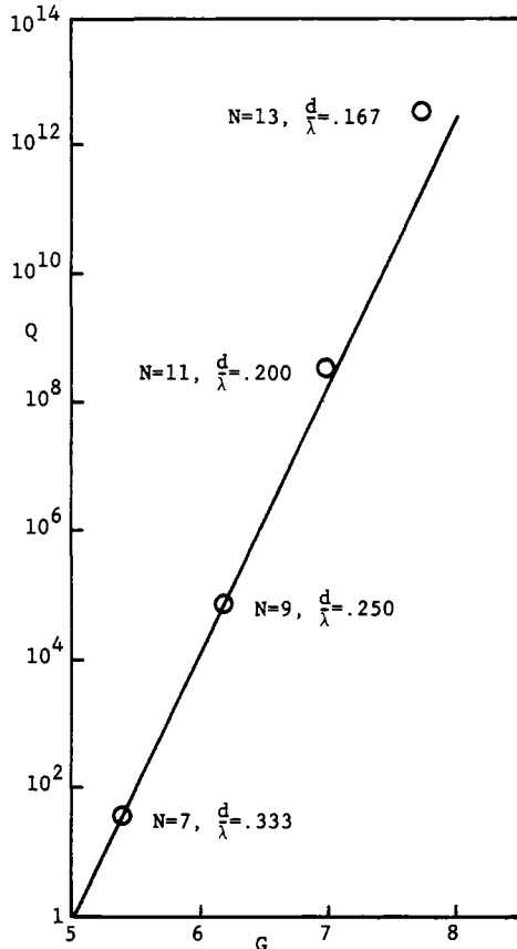
Fig. 5. Q versus directivity, 10 dB SLR, array length 2λ.
