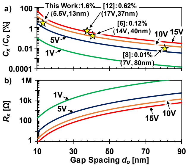
Fig. 2: Simulated plots of (a) electromechanical coupling strength ( C_x/C_o ) and (b) motional resistance R_x versus electrode-to-resonator gap spacing d_o and bias voltage V_P for a 2\mu\text{m} -thick 60-MHz wineglass disk resonator with Q=70,000 .
