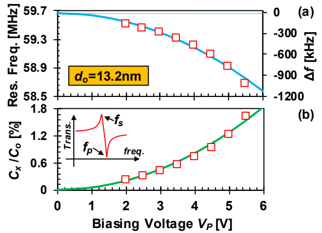
Fig. 9: 10 \mu Torr-vacuum-measured (a) resonance frequency and (b) electromechanical coupling (C_x/C_o) for a 13.2nm-gap WG disk determined using series f_s and parallel f_p resonance frequencies, both plotted against bias voltage V_P .
