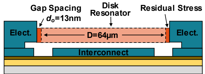
Fig. 4: Illustration depicting how residual stress can cause shorts between disk and electrode when the gap becomes very small.
