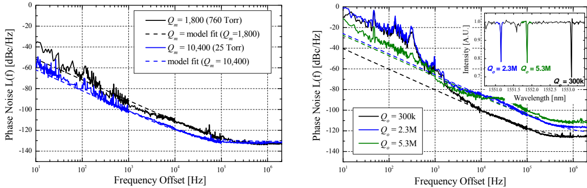
Fig. 2 (a) Fitted and measured phase noise of 25µm outer radius nitride OMO with f_m=74 MHz (b) Measured and model fit (dashed) phase noise for three optical resonances in the same 50µm PSG device. Inset: three optical resonances seen in transmission through tapered fiber.
