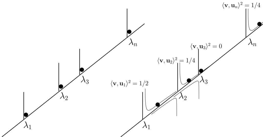
Figure 1: Physical model of interlacing eigenvalues.
