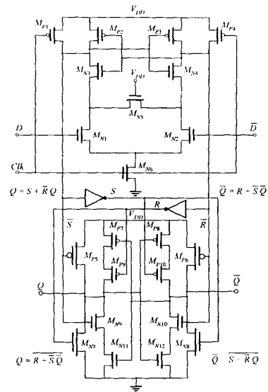
Figure 16.5.2: Modified sense amplifier-based flip-flop.
