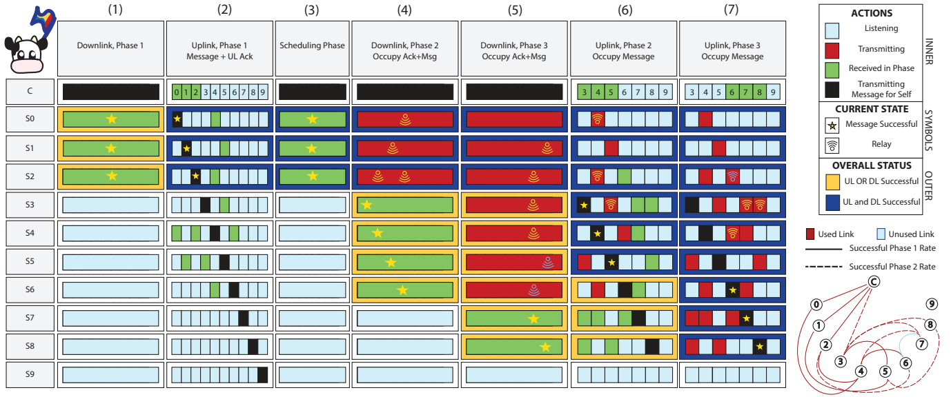
Fig. 1. The seven phases of the Occupy CoW protocol illustrated by a representative example. The table shows a variety of successful downlink and uplink transmissions using 0, 1 or 2 relays. S9 is unsuccessful for both downlink and uplink. The graph on the right shows the underlying link-strengths for the network.
