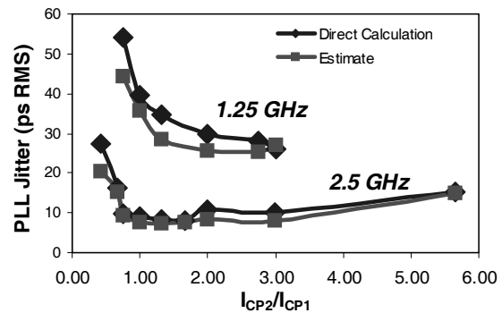
Figure 13: PLL jitter at various operating points for two different operating frequencies.
