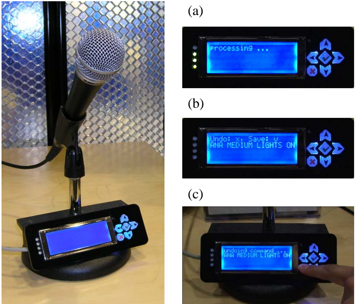
Figure 5.1: Next to each microphone there is a small display which contains an LCD, four vertical LEDs and five buttons. The LEDs show the volume of the microphone (a). The LCD shows “processing ...” if the system is processing an audio command (a) and then shows the output of the automatic speech recognizer (b). The user can undo the effect of the last command if necessary by pushing the button labeled “x” (c).
