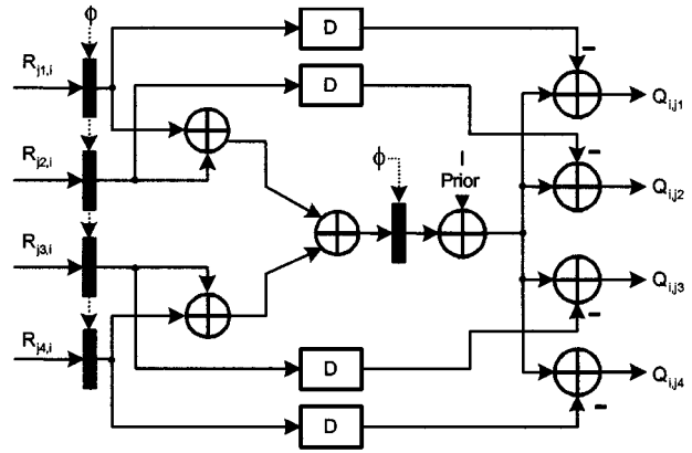
Fig. 15. Binary adder tree to compute bit-to-check message in a 2-stage pipeline.
