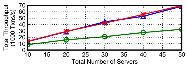
Figure 6: Scale-out of MAV, Eventual, and RC.
