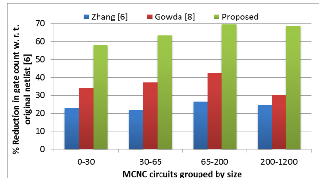
Figure 2 – Percentage gate count reduction in each approach, compared to the original netlist [6].
