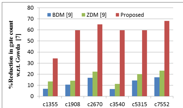
Figure 3 – Percentage gate count reduction in each approach, compared to Gowda [8].
