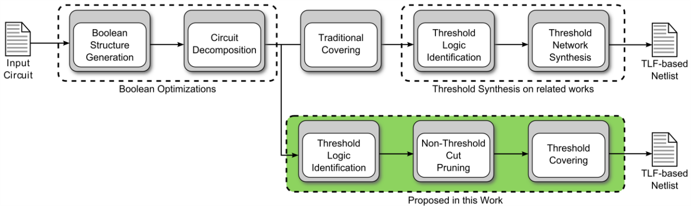
Figure 1: Threshold logic synthesis flow proposed in this work.
