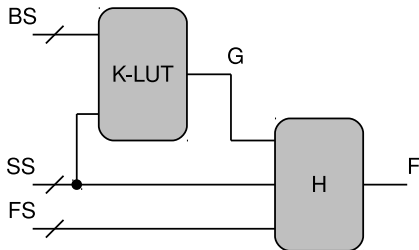
Fig. 4. Illustration of the Roth-Karp decomposition technique used to create LUT structures for logic functions.
