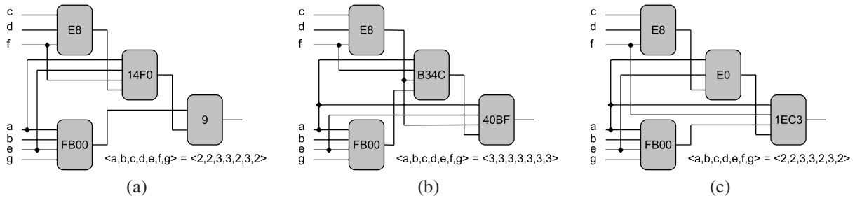
Fig. 5. Example of pruning LUT structures using timing profiles. Assume that structure (a) has already been computed. Structure (b) is rejected because its timing profile is worse than that of (a). Structure (c) is rejected as well because its timing profile is equal to that of (a) and its area is not better than (a). Neither structure (b) nor (c) offer any benefit in performance or area over (a).
