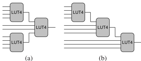
Fig. 1. Examples of LUT structures consisting of three 4-LUTs which are suitable for implementing many logic functions of up to 10 inputs.
