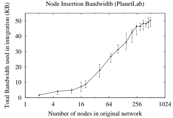
Fig. 17. Node Insertion Bandwidth . Total control traffic bandwidth for single node insertion.
