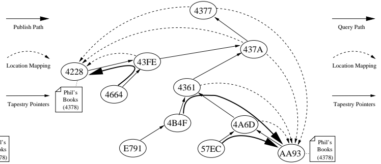
Fig. 5. Tapestry route to object example. Several nodes send messages to object 4378 from different points in the network. The messages route towards the root node of 4378. When they intersect the publish path, they follow the location pointer to the nearest copy of the object.
