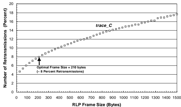
Figure 7: Number of Retransmissions versus Frame Size.
