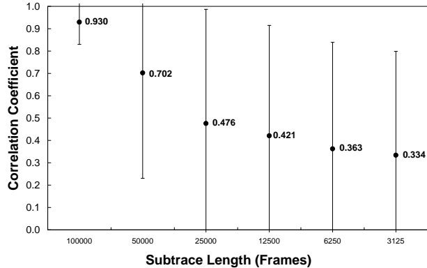
Figure 10. WLAN_E error path modeling: mean and standard deviation correlation coefficient values for different subtrace lengths.
