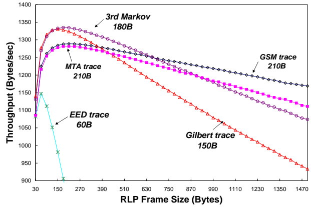
Figure 1. Optimal frame size versus error model.
