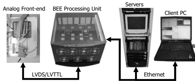
Figure 1: BEE emulation system overview
