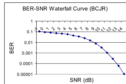
Figure 8: Measured BCJR decoder waterfall curve
