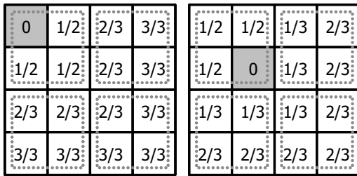
Figure 3: Inter-FPGA connection hop counts
