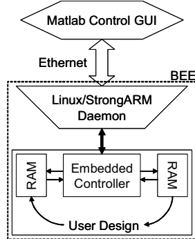
Figure 4: Hardware-in-the-loop data I/O interface
