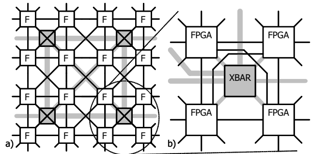
Figure 2: BEE interconnect structure, a) all twenty FPGAs and b) detailed routing in one board quadrant, emphasizing the nature of crossbar FPGAs
