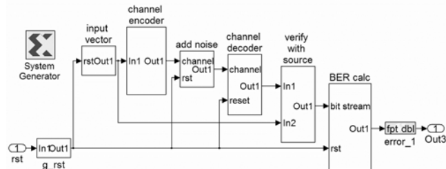
Figure 7: Turbo decoder design in Simulink
