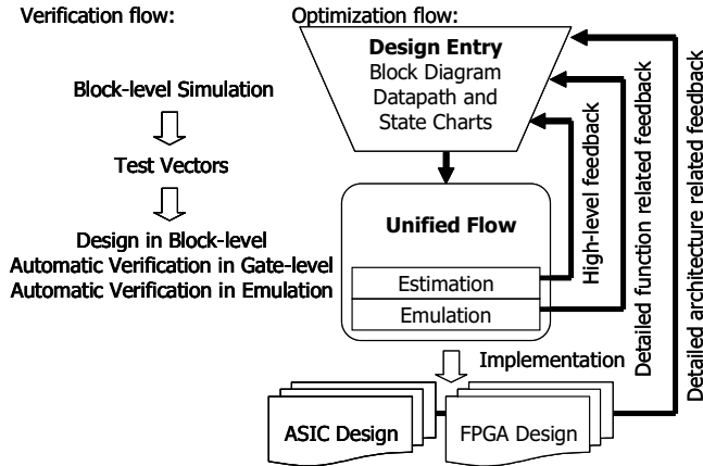
Figure 5: BEE design verification and optimization flows
