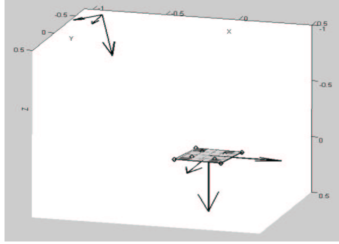
Figure 10. Reconstruction result for the translational symmetry. The structure is represented in the canonical world coordinate frame. From our discussion above, the origin o of the world coordinate may translate freely within the xy -plane. The smaller coordinate frame is the camera coordinate frame. The longest axis is the z -axis of the camera frame which represents the the optical axis of the camera.
