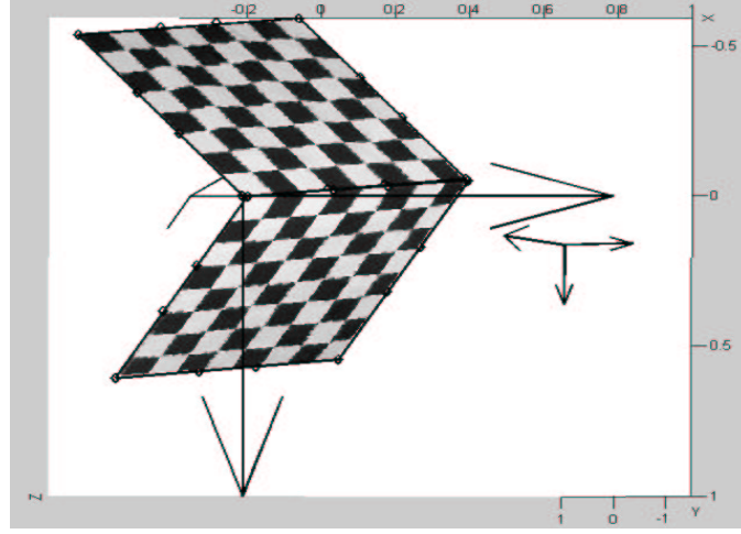
Figure 8. Reconstruction result from the rotational symmetry. The recovered structure is represented in the canonical world coordinate frame. From our discussion above, the origin o of the world coordinate may translate freely along the z -axis, and the x, y -axis can be rotated within the xy plane freely. The smaller coordinate frame is the camera coordinate frame. The longest axis is the z -axis of the camera frame which represents the the optical axis of the camera.
