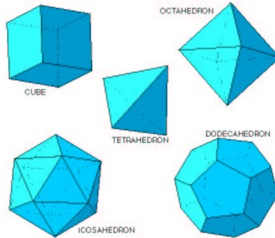
Figure 19. Five Platonic solids.
