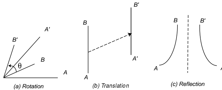
Figure 17. The three basic types of isometric transformations.
