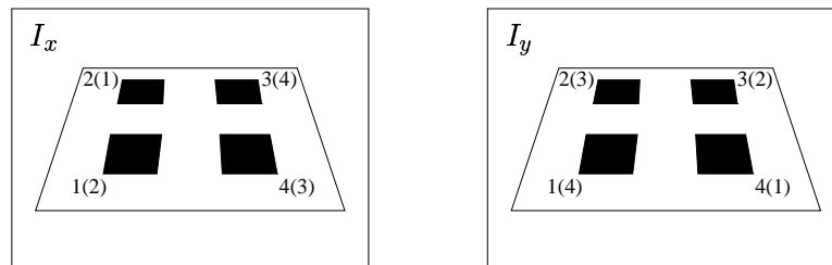
Figure 3. I_x : Corner correspondence between the original image of the board and an “image” with the board reflected in the x -axis by 180^\circ ; I_y : Corner correspondence between the original image of the board and an “image” with the board reflected in the y -axis by 180^\circ .
