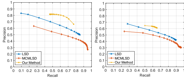
Figure 6. The precision-recall curves of different line segment detection methods. Left: on our test dataset. Right: on the York Urban dataset [7].
