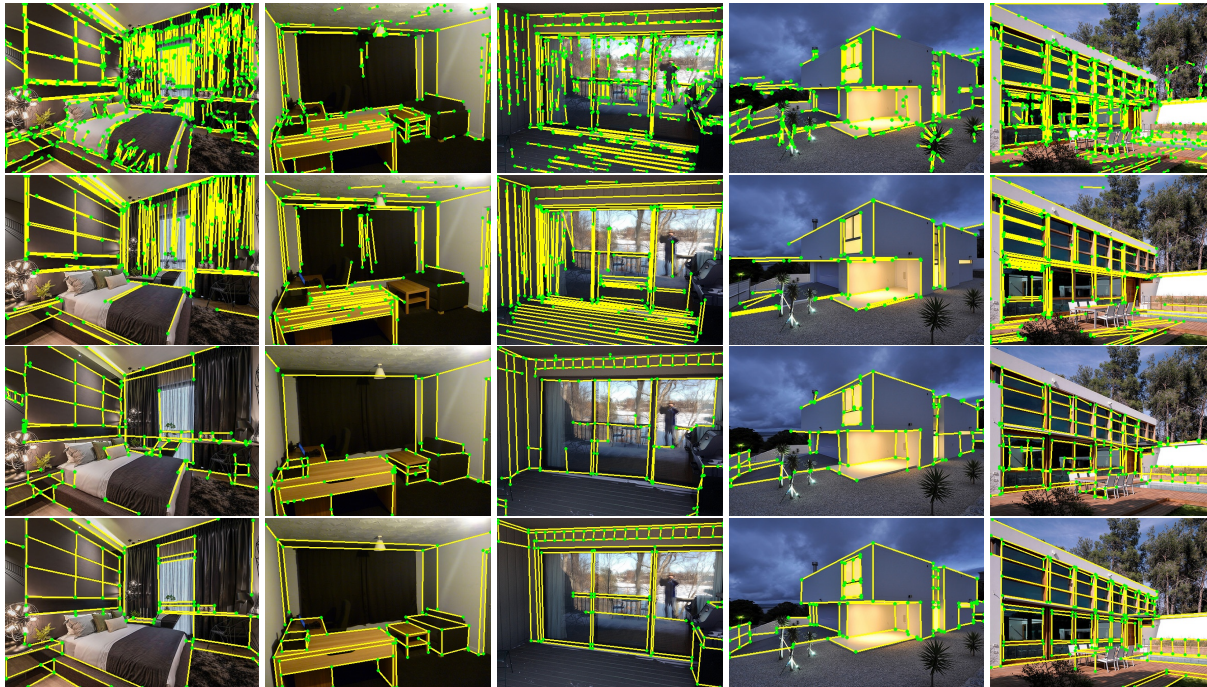
Figure 8. Line/wireframe detection results. First row: LSD ( -\log(\text{NFA}) > 0.01 * 1.75^8 ). Second row: MCMLSD (confidence top 100). Third row: Our method (line heat map h(p) > 10 ). Fourth row: Ground truth.
