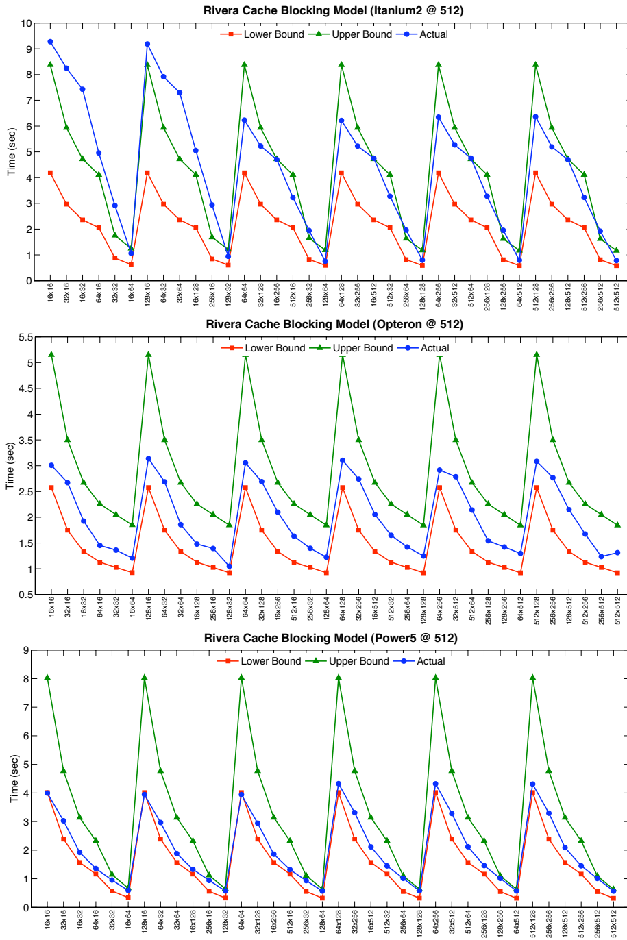
FIG. 4.2. Comparison between partial 3D-blocking runs and the lower/upper bounds of our memory model. Results show that our analytical approach is extremely effective in predicting blocked stencil performance.
