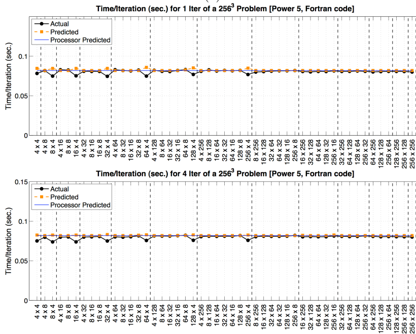
FIG. 6.3. A comparison of the time skewing performance model against reality on non-Itanium architectures. The graphs show running times on the (a) Opteron and (b) Power 5 for a 256^3 problem with constant boundaries. In both pairs of graphs, the top graph shows data for one iteration, while the bottom graph shows average data over four iterations. On all graphs, the x-axis shows the x and y-dimensions of each plotted cache block size (the z-dimension, which is contiguous in memory, is not shown because it is always uncut). The x-axis is ordered such that the block sizes are monotonically increasing, and the vertical dotted lines divide areas of equal-sized cache blocks.
