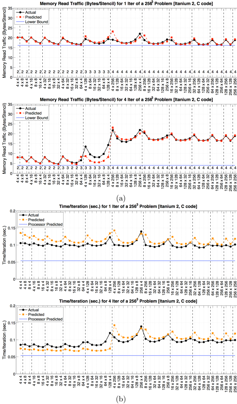
FIG. 6.2. A comparison of the time skewing performance model against reality on the Itanium2. The graphs show (a) main memory read traffic and (b) running times for a 256^3 problem with constant boundaries. In both pairs of graphs, the top graph shows data for one iteration, while the bottom graph shows average data over four iterations. On all graphs, the x-axis shows the x and y-dimensions of each plotted cache block size (the z-dimension, which is contiguous in memory, is not shown because it is always uncut). The x-axis is ordered such that the block sizes are monotonically increasing, and the vertical dotted lines divide areas of equal-sized cache blocks.
