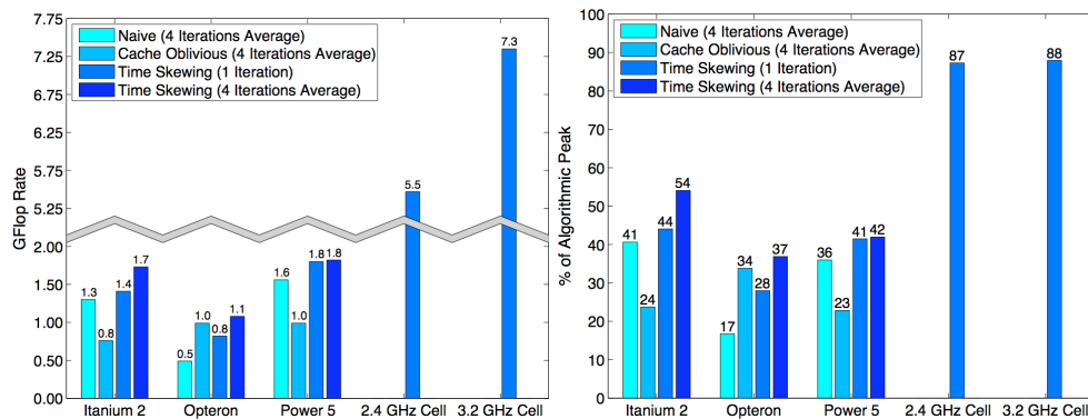
FIG. 9.1. (left) GFlop rates and (right) percentage of algorithmic peak, for a 256^3 problem with constant boundaries. “Time Skewing (1 Iteration)” data is essentially space-only cache blocking.
