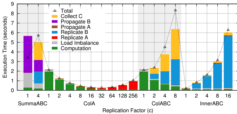
Fig. 5: Cost breakdown for multiplying a square Erdős-Rényi matrix of size n = 65,536 with 41 nonzeros per row with a dense matrix of same size on p = 3,072 cores of Cray XC30 (256 MPI processes). All three 1.5D algorithms outperform SummaABC with ColA having the lowest communication time and also the best total running time. Only SummaABC moves the dense B matrix, so it is the slowest as expected.
