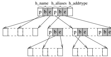
Fig. 3. Representation of struct hostent after the CCured transformation. Array-bounds metadata (gray) is interspersed with data (white).
