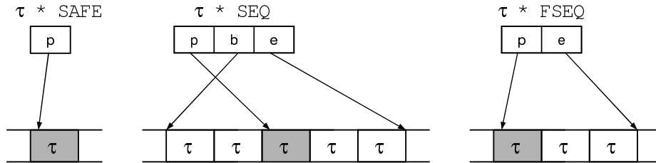
Fig. 1. SAFE, SEQ and FSEQ pointers, respectively, to the shaded memory locations.
