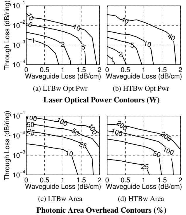
Figure 6: Laser Optical Power and Area Overhead Contours for 64 \times 64 CMXbar – Systems implemented with serpentine layout on 20 \times 20 mm die.
