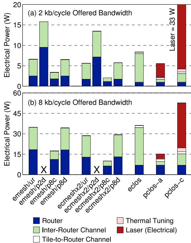
Figure 12: Dynamic Power Breakdown – Power of eclos and pclos did not vary significantly across traffic patterns. (a) LTBw systems at 2 kb/cycle offered bandwidth (except for emesh/p2d and ecmeshx2/p2d which saturated before 2 kb/cycle, HTBw system shown instead), (b) HTBw systems at 8 kb/cycle offered bandwidth (except for emesh/p2d and ecmeshx2/p2d which saturated before 8 kb/cycle).
