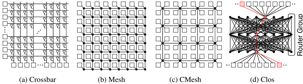
Figure 1: Logical View of 64 Tile Network Topologies – (a) 64x64 distributed tristate global crossbar, (b) 2D 8x8 mesh, (c) concentrated mesh (cmesh) with 4x concentration, (d) 8-ary, 3-stage Clos network with eight middle routers. In all four figures: squares = tiles, dots = routers, triangles = tristate buffers. In (b) and (c) inter-dot lines = two opposite direction channels. In (a) and (d) inter-dot lines = uni-directional channels.
