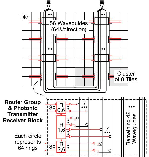
Figure 8: U-Shaped Layout for 8-ary 3-stage Clos – Electrical circuitry shown in red. 56 waveguides ( 8 \text{ sets of } 7 ) are either routed between columns of tiles (monolithic integration) or over tiles (3D integration). Each of the 8 clusters (8 tiles per cluster) has electrical channels to its router group which contains one router per Clos stage. In the inset, the first set of 7 waveguides are used for channels (each 64 \lambda = 128 \text{ b/cycle} ) connecting to and from every other cluster. The second set of 7 waveguides are used for the second half of the Clos network. The remaining 42 waveguides are used for point-to-point channels between other clusters.
