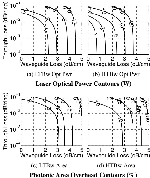
Figure 9: Laser Optical Power and Area Overhead Contours for 8-ary 3-stage Clos – Systems implemented with U-shaped layout on 20 \times 20 mm die.
