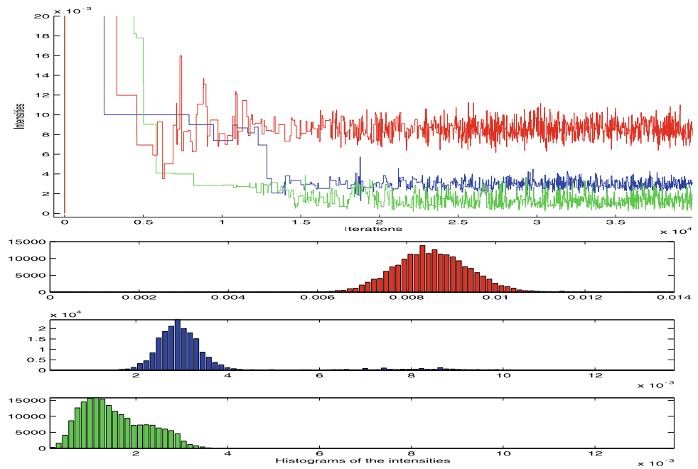
Fig. 5 Top: Trace of the intensities h_0, h_1, h_2 for k = 2 corresponding to iterations 1, \dots, 40,000 . Bottom: Histogram of the intensities for k = 2 after 200,000 iterations (with the first 10,000 samples discarded)
