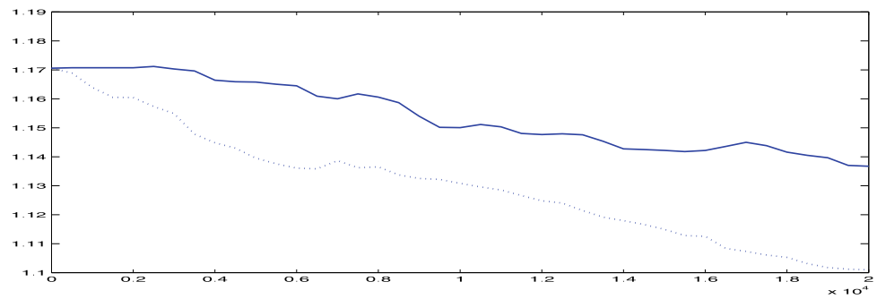
Fig. 2 Comparison of the R coefficient for the standard AM algorithm ( top ) and the multi-criteria algorithm ( bottom ) as a function of the iterations
