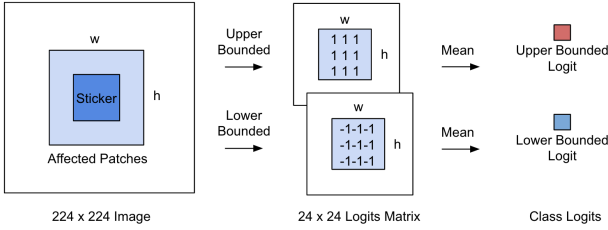
Fig. 4. Computing upper and lower bounds on logits, for certified security.
