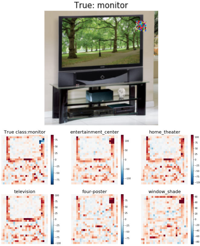
Fig. 3. An image from ImageNet with an adversarial sticker, and the heatmaps produced by BagNet-9. In this case the attack is successful: the true class is not among the top 5 predictions.
