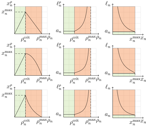
Figure 2: Examples of flux functions for horizontal queues (left) and corresponding latency as a function of the density \ell_n^\rho(\rho_n) (middle) and as a function of the flow and the congestion state \ell_n(x_n, m_n) (right). The free-flow (respectively congested) regime is shaded in green (respectively red).
