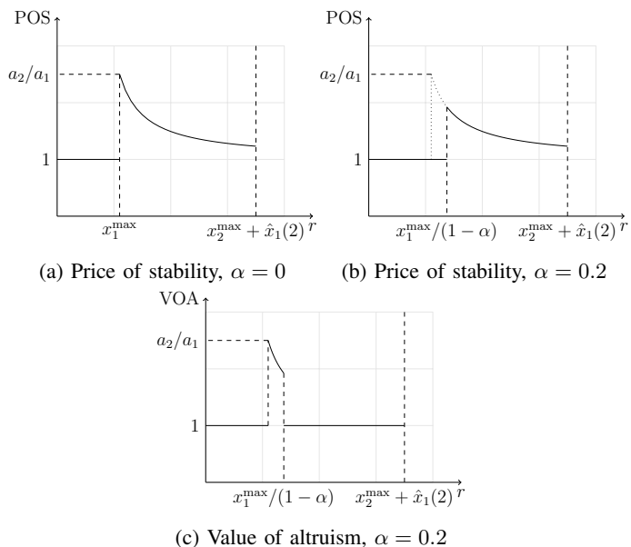
Figure 9: Price of stability and value of altruism on a two-link network. Here we assume that \hat{x}_1(2) + x_2^{\max} > x_1^{\max} .
