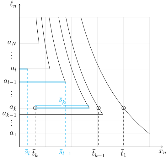
Figure 5: Non-compliant first (NCF) strategy \bar{s} and its induced equilibrium. Circles show the best Nash equilibrium (\bar{t}, \bar{m}) of the non-compliant flow (1 - \alpha)r : link \bar{k} is in free-flow, and links \{1, \dots, \bar{k} - 1\} are congested. The Stackelberg strategy \bar{s} = \text{NCF}(N, r, \alpha) is highlighted in blue.
