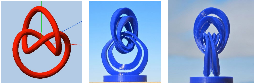
Fig. 5: (a) Trefoil knot with D_2 symmetry. (b,c) A “2-lobe” version of a Trefoil cable-knot, two views.
