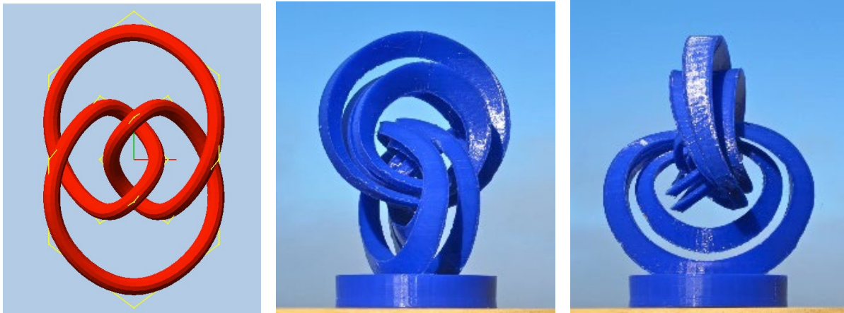
Fig. 7: (a) 2-lobe layout of the Figure-8 knot. (b,c) A 2-lobe variant of the Figure-8 cable-knot.
