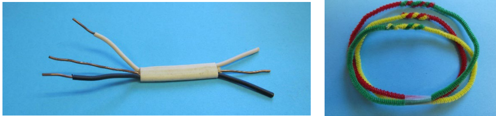
Fig. 2: (a) A 3-strand “Cable.” (b) Closing a twisted cable into a single-strand loop.
