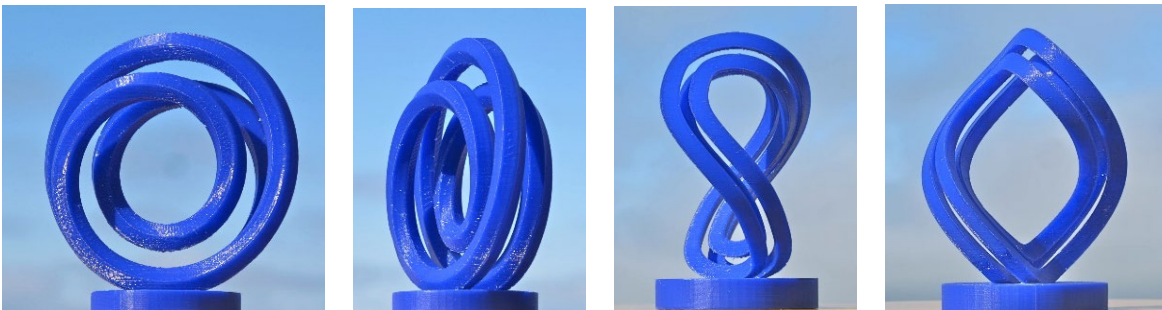
Fig. 3: Unknots: (a,b) A simple torus knot, front and side. (c,d) Warped version of the same knot.
