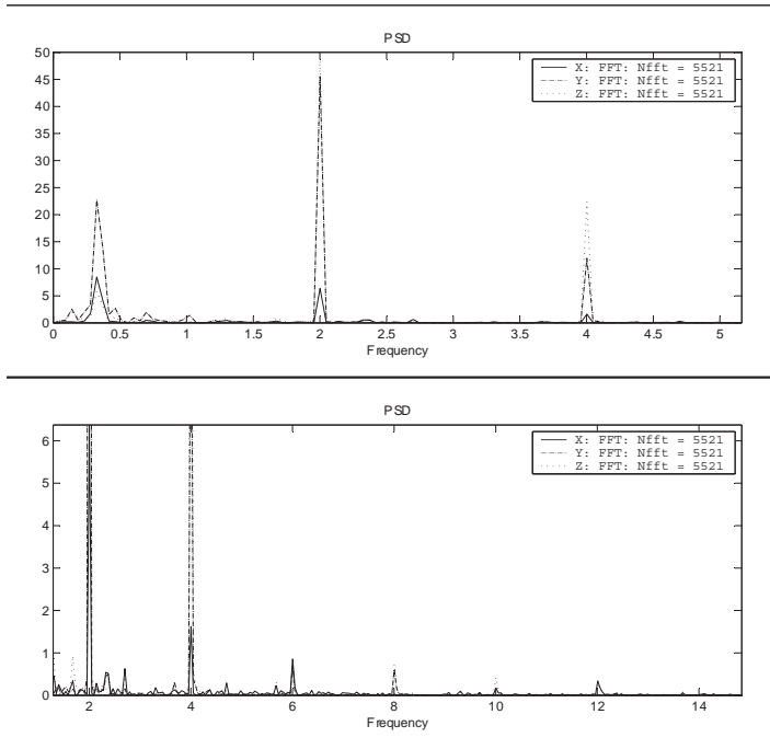
Fig. 4. Power spectral density (PSD) of the motion of the point-of-interest. The x, y, and z components of the motion are superimposed to better show the dominant modes, which are at 0.37 Hz and 2.0 Hz. Note the change in scales between the low frequency range (top), and the moderate-to-high frequency range (bottom).
