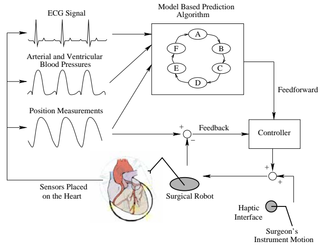
Fig. 2. The proposed control architecture for Active Relative Motion Cancellation
