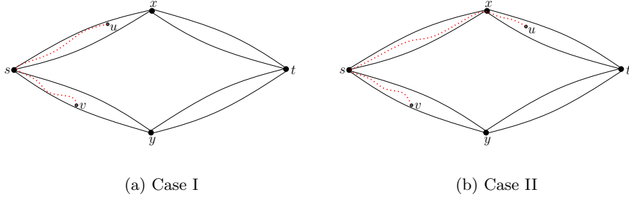
Figure 2: The two cases of Theorem 5.1
