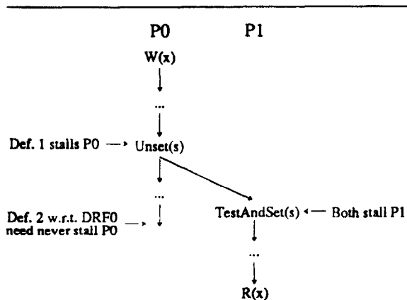
Figure 3. Analysis of the new implementation.
