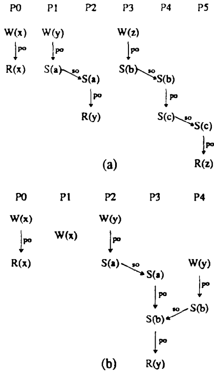
Figure 2. An example and counter-example of DRF0.
