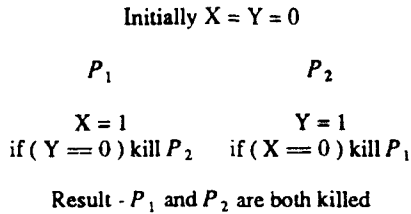
Figure 1. A violation of sequential consistency.
