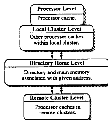
Figure 2. Logical memory hierarchy of DASH.
