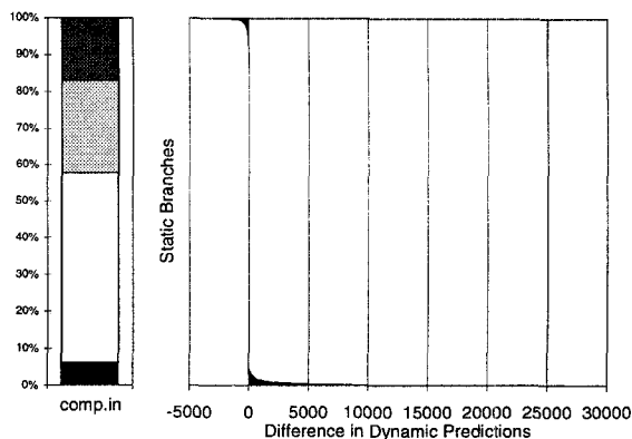
Figure 15. Detailed information on the comp.in bar from Figure 14. The horizontal axis shows the difference in correct predictions by the static and 2-bit counter predictors. Positive values correspond to the 2-bit counter predicting more accurately; negative values correspond to the static predictor predicting more accurately.
