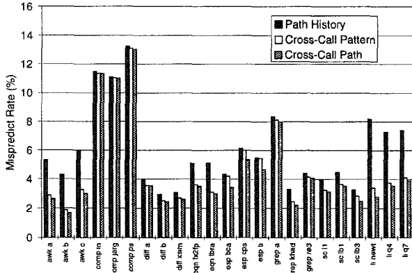
Figure 12. Mispredict rates of schp using path history (same as the third series in Figure 6) and simulated mispredict rates for cross-call pattern and cross-call path history dividers with static predictors. These results use a history depth of 12 and train and test on the same dataset.
