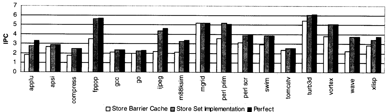
Figure 6.7: Final Store Set Implementation vs. Perfect
