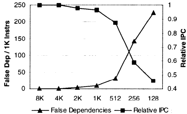
Figure 6.5: Fpppp - Performance vs. Number of Entries in SSIT
