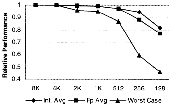
Figure 6.4: Performance Sensitivity to Number of Entries in SSIT
