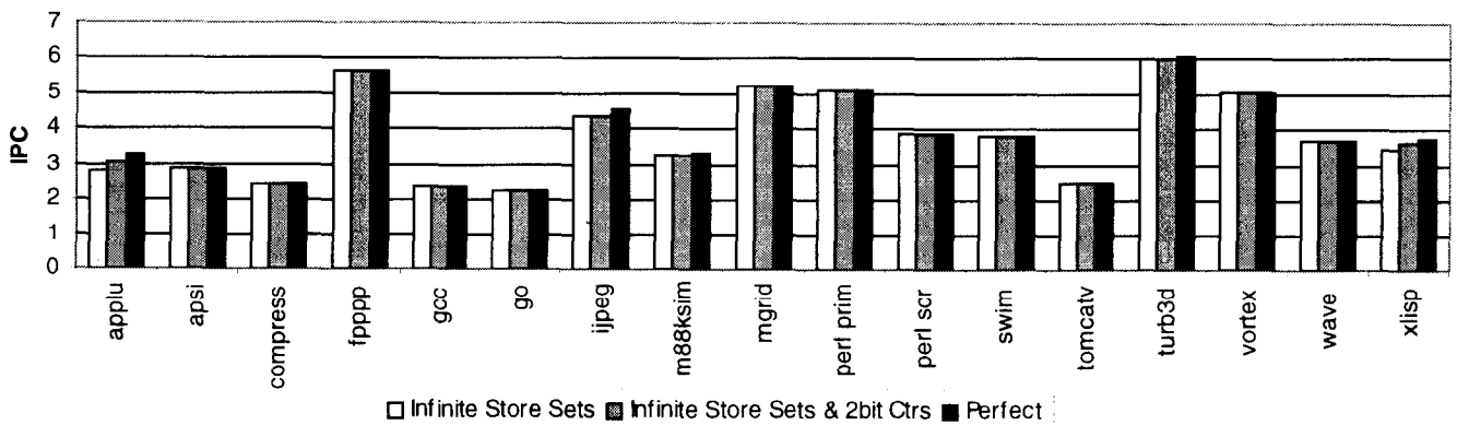
Figure 5.4: Performance of Store Set Memory Dependence Prediction
