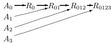
FIG. 2.4. Graphical representation of sequential TSQR.
