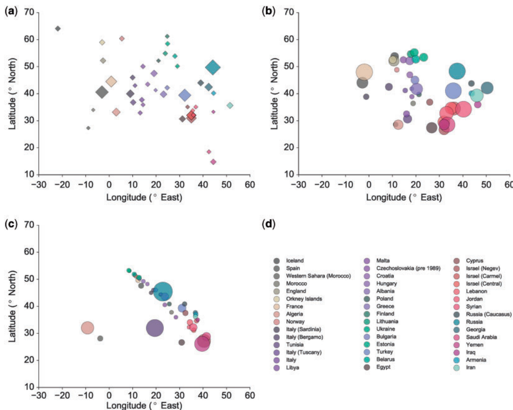
Fig. 2. PCA and GAP visualization of the North African and West Eurasian samples in the Human Origins dataset. Each data point corresponds to the sampling location of a population. (a) True sampling locations, (b) GAP reconstructed locations, (c) PCA reconstructed locations and (d) population legends. The areas of the circles are proportional to the estimated variance in the reconstructed locations of the samples in each subpopulation, while the areas of the diamonds are proportional to the number of sampled individuals from the population (Color version of this figure is available at Bioinformatics online.)
