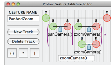
Figure 1. Proton represents a gesture as a regular expression describing a sequence of touch events. Using Proton’s gesture tablature, developers can design a multitouch gesture graphically by arranging touch sequences on horizontal tracks. Proton converts the tablature into a regular expression. When Proton matches the expression with the touch event stream, it invokes callbacks associated with the expression.
