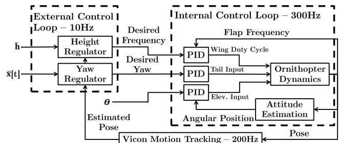
Fig. 3. Block diagram of the H 2 Bird control system.
