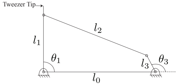
(a) Idealized model of four bar gripper
