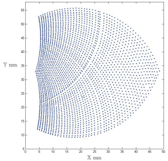
Fig. 11. Approx. 2500 experimentally sampled task space output positions resulting from uniform actuator inputs in increments of 1.8^\circ .
