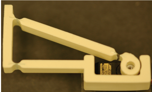
(b) Compliant four bar finger linkage with servo motor actuator attached
