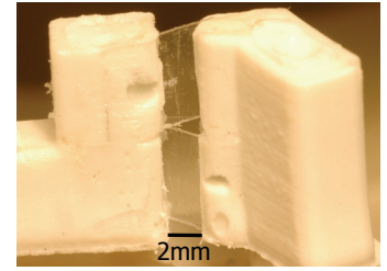
(b) Crossed strip flexure hinge (w/ PET flexures) integrated into manipulator
